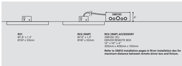
CEILING 4803-S-32
